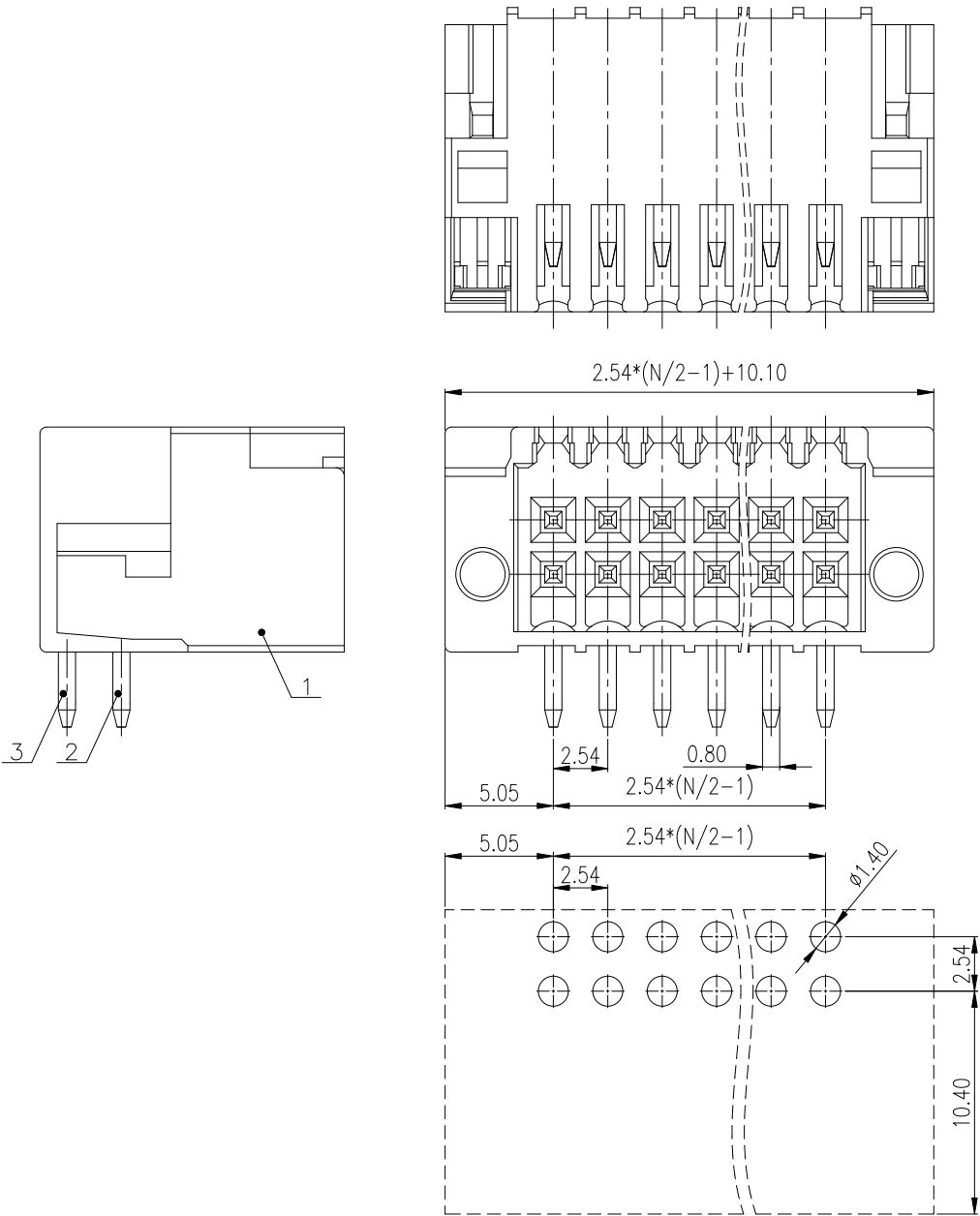
PCB LAYOUT
